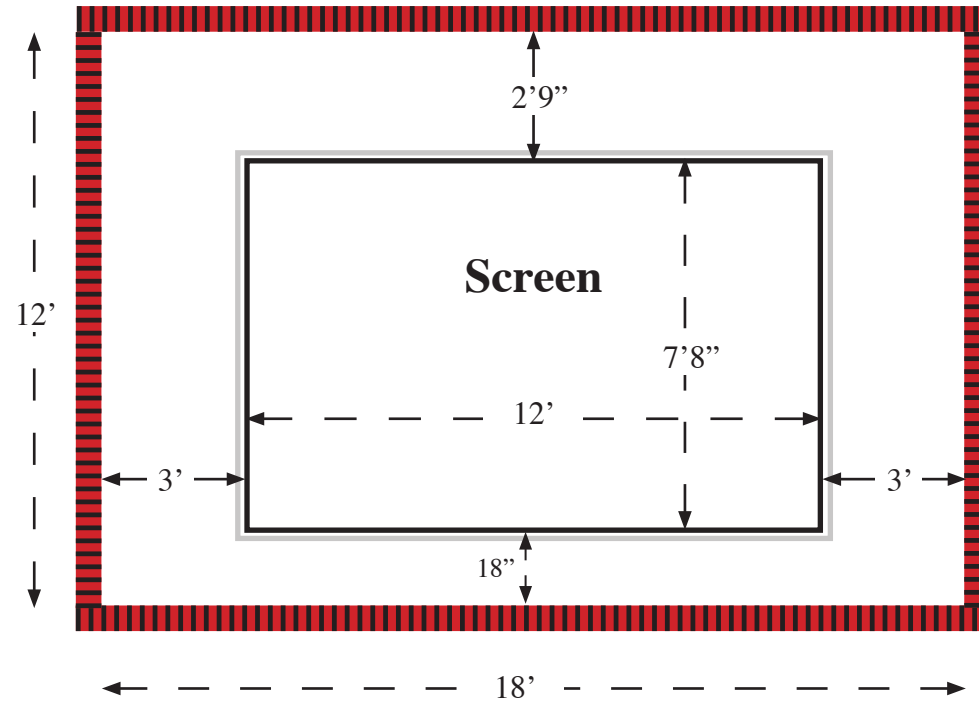
Front Wall (Screen)
