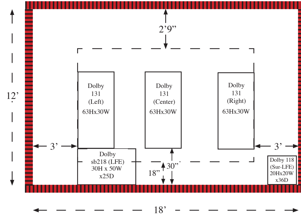
Front Wall (Speakers)
