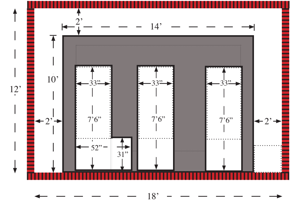
Front Wall (Cutouts)
